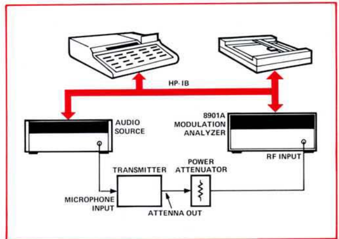
Figure 6-8. Automatic transmitter test equipment setup.
