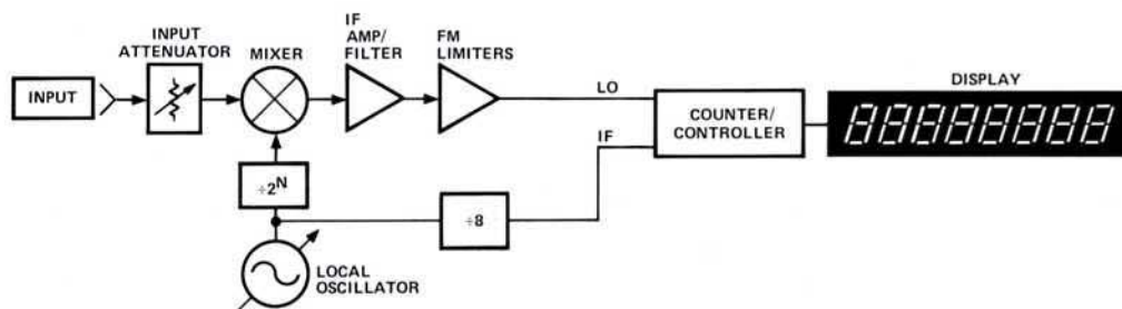
Figure 4-1. Input frequency measurement block diagram.
