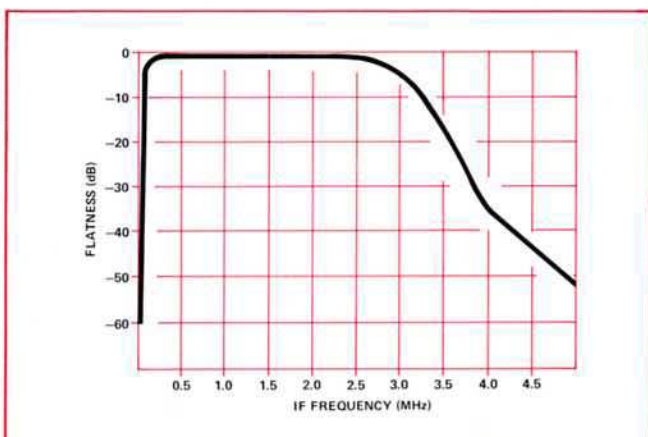
Figure 4-23. 1.5 MHz IF filter characteristic.
