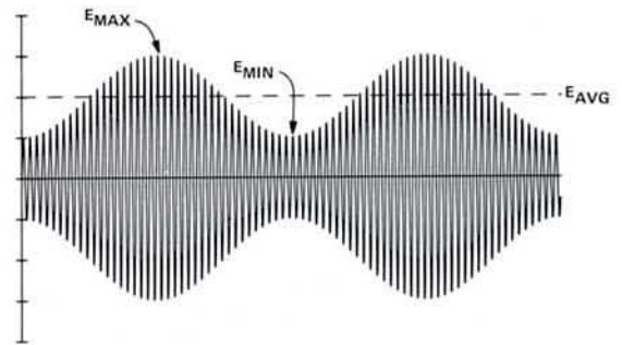
Figure 5-4. RF carrier modulated with 50% AM.
