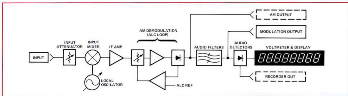
Figure 4-3. AM measurement block diagram.
