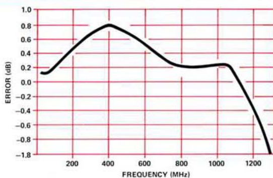
Figure 4-17. Typical 8901A RF level accuracy.
