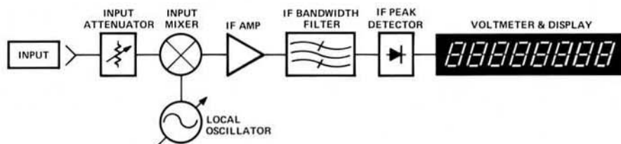
Figure 4-18. Tuned RF level measurement block diagram.
