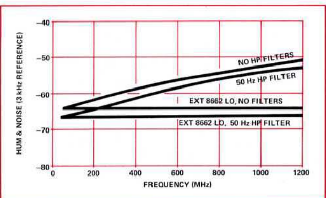
Figure 4-10. Typical 8901A hum & noise (750 μs pre-display mode).
