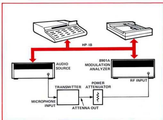
Figure 2-3. Automated FM transmitter testing
